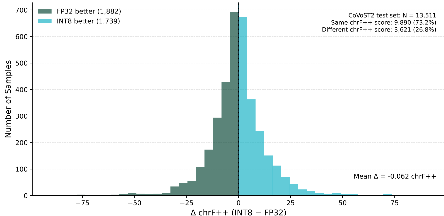
Distribution of FP32-INT8 chrF++ Differences
