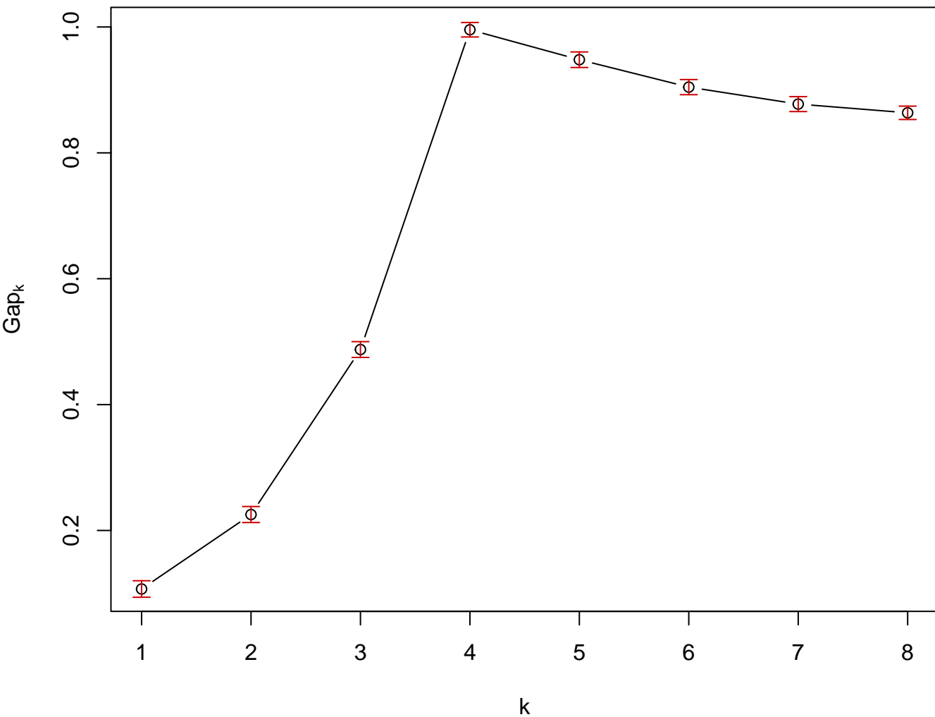
Gap statistic (hypercube demo)
