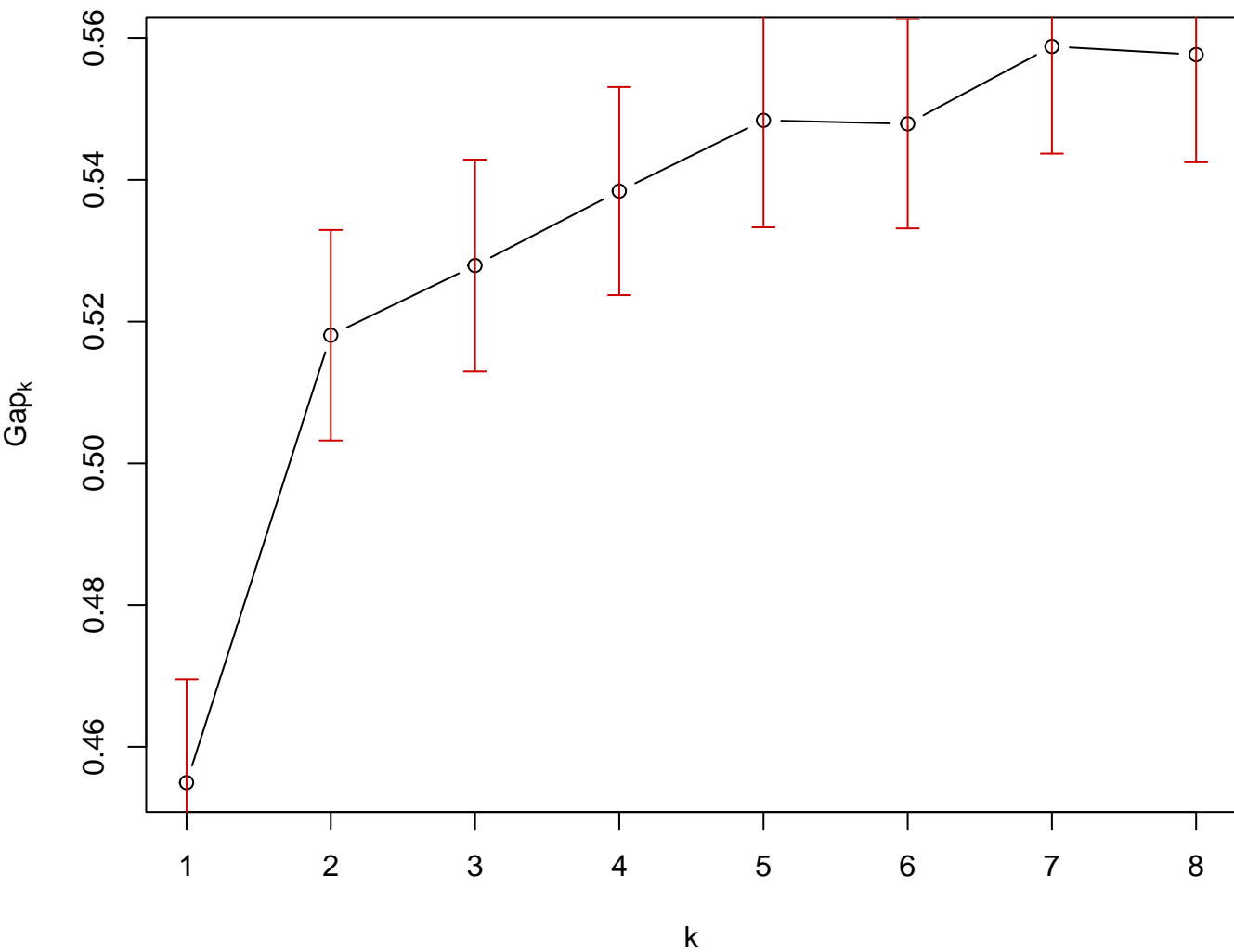
Gap statistic (spectral on shells)
