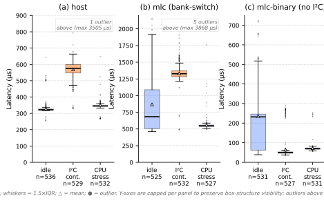
Fig. 1. Per-trial wire-level latency by pipeline and condition. The mlc-binary panel (zero I 2 C transactions on the decision path) isolates the kernel/gpioid latency floor; note the per-panel y-axis scaling.
