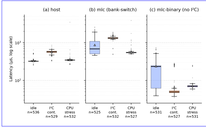
Fig. 1. Per-trial wire-level latency by pipeline and condition, on one shared log-scale y-axis across all three panels so box position is directly comparable across pipelines . The mlc-binary panel (zero I 2 C transactions on the decision path) isolates the kernel/gpio latency floor; note the per-panel y-axis scaling . Box = IQR (Q1–Q3); whiskers = 1.5×IQR; \Delta = mean; \bullet = outlier; y-axes are capped per panel every point is shown in-frame, with outliers above each cap noted in-panel no per-panel capping .
