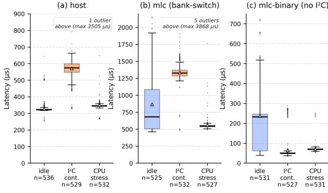
Fig. 1. Per-trial wire-level latency by pipeline and condition. The mlc-binary panel (zero I 2 C transactions on the decision path) isolates the kernel/gpid latency floor; note the per-panel y-axis scaling. Box = IQR (Q1–Q3); whiskers = 1.5×IQR; \Delta = mean; \bullet = outlier; y-axes are capped per panel, with outliers above each cap noted in-panel.
