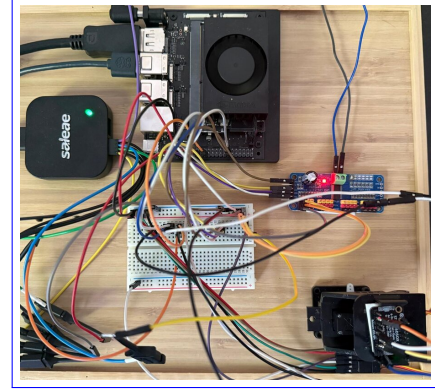
Fig. 2. Measurement setup. The LSM6DSOX IMU (on a servo-driven motion stimulus) and the PCA9685 servo controller connect to the NVIDIA Jetson Orin Nano over separate I²C buses; a Saleae Logic Pro 8 taps the sensor INT1 edge (D0), the host decision GPIO (D1), and the servo PWM command (D2) for wire-level timing.
