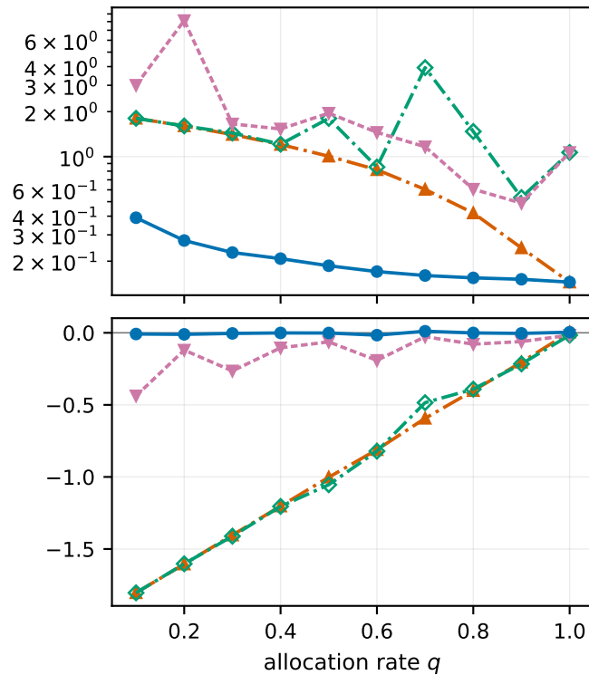
Amazon
