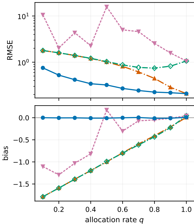
Synthetic
