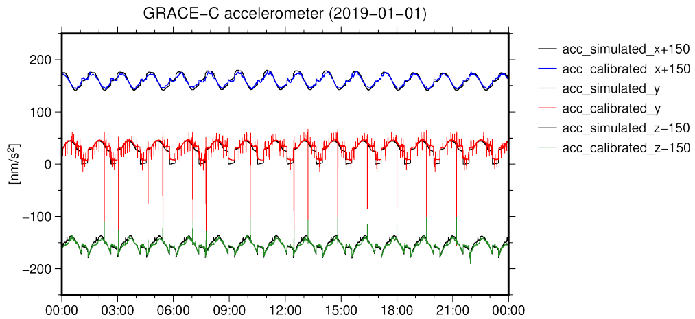
Figure 3.3: Example 3: Calibrating GRACE-C ACT1B data.
