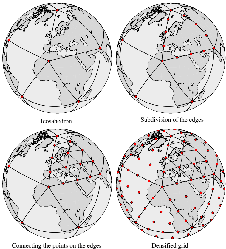
Figure 5.7: TriangleVertex grid.
