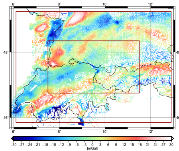
Figure 3.9: Gravity disturbances: observed minus computed
