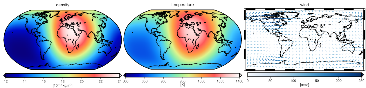
Figure 4.19: JB2008 model in 300 km height at 2003-07-01 12:00.
