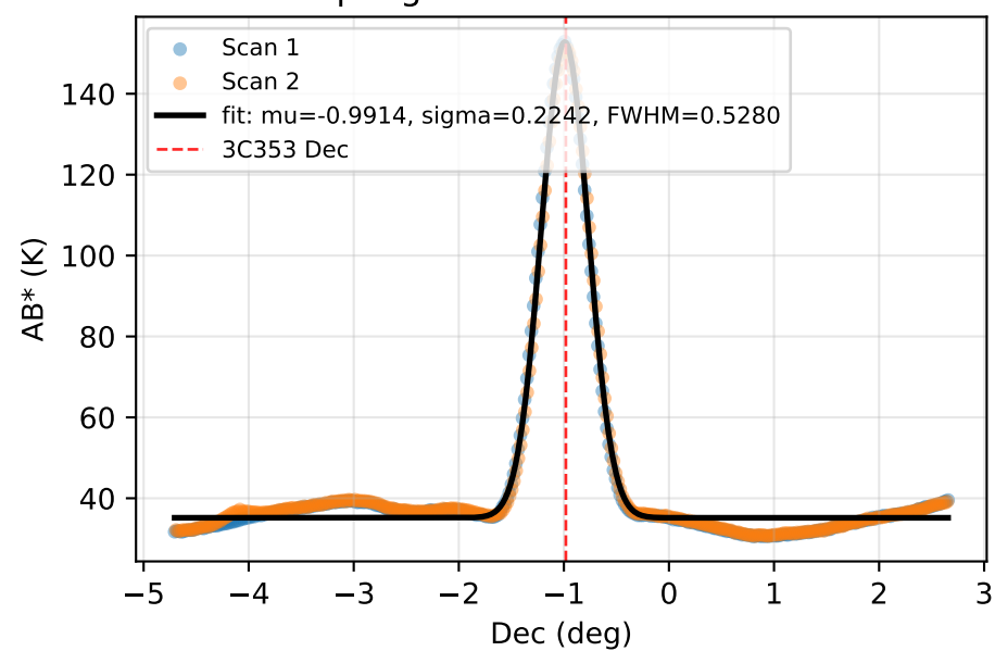
Freq-avg: Gaussian fit across Dec
