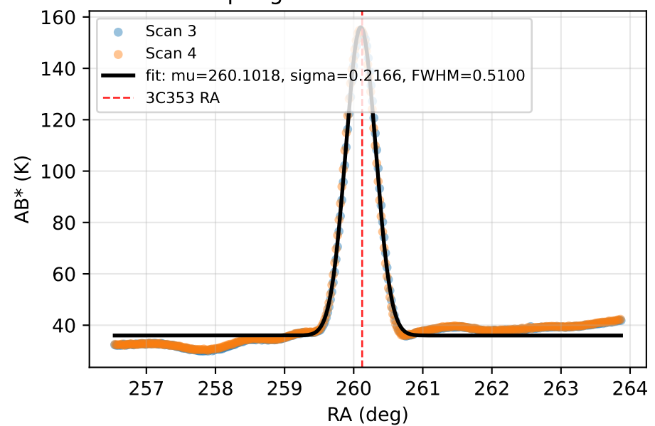
Freq-avg: Gaussian fit across RA
