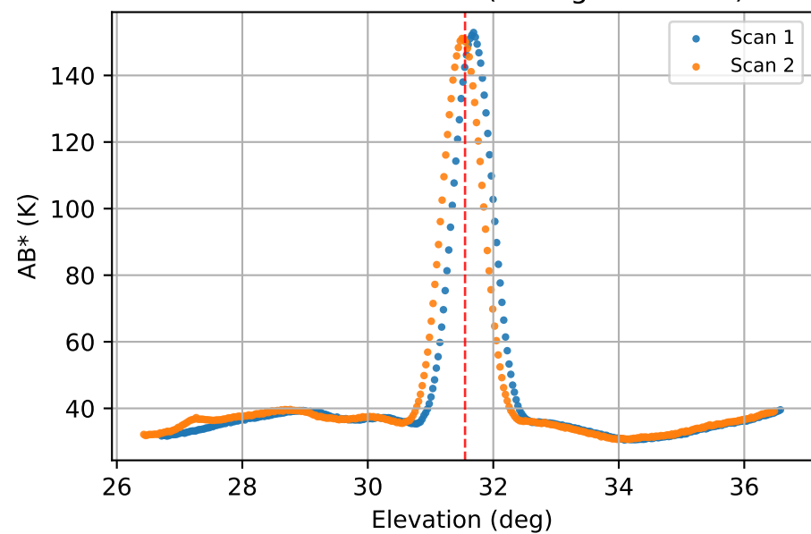
Peak Scan: Elevation (timing-corrected)
