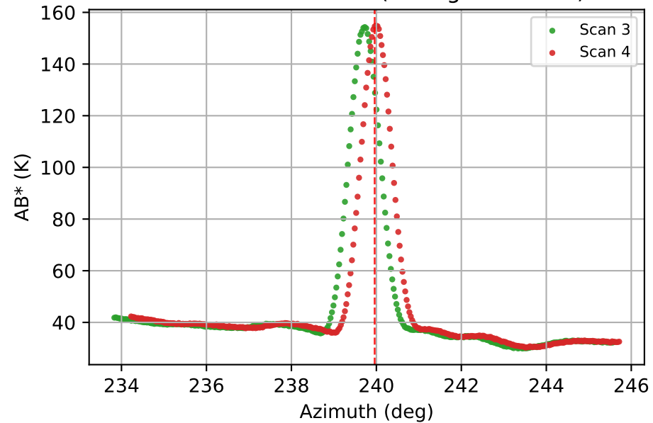
Peak Scan: Azimuth (timing-corrected)
