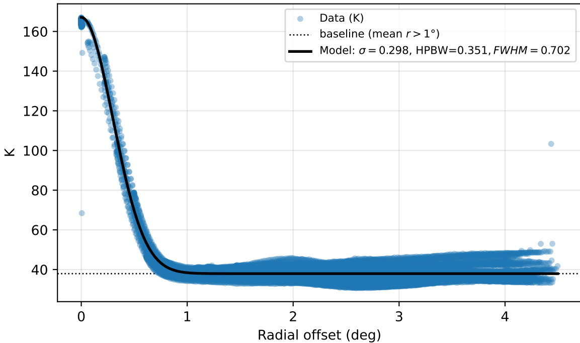
Beam profile
