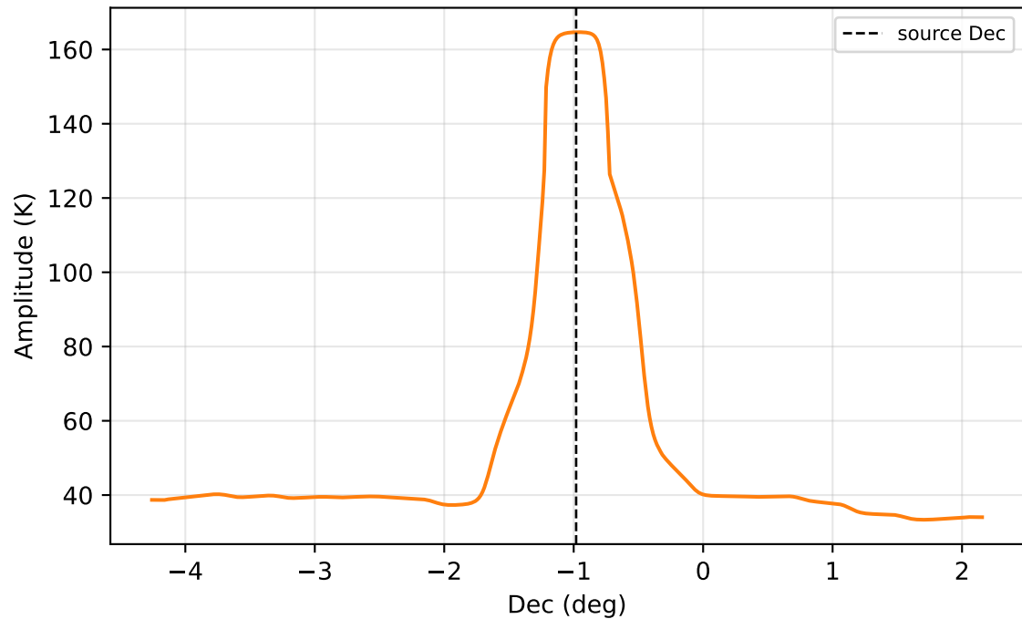
Scan across source (fixed RA = 260.121^\circ )
