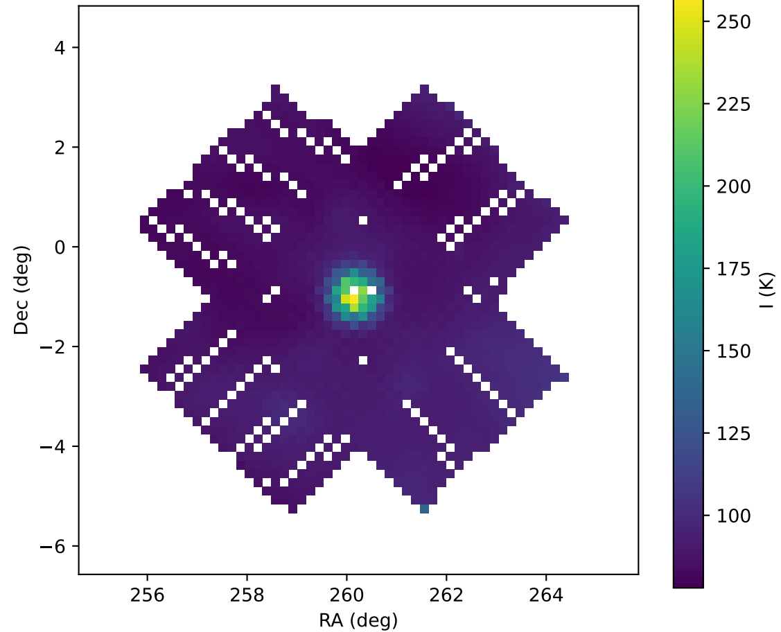
Dirty Stokes I
