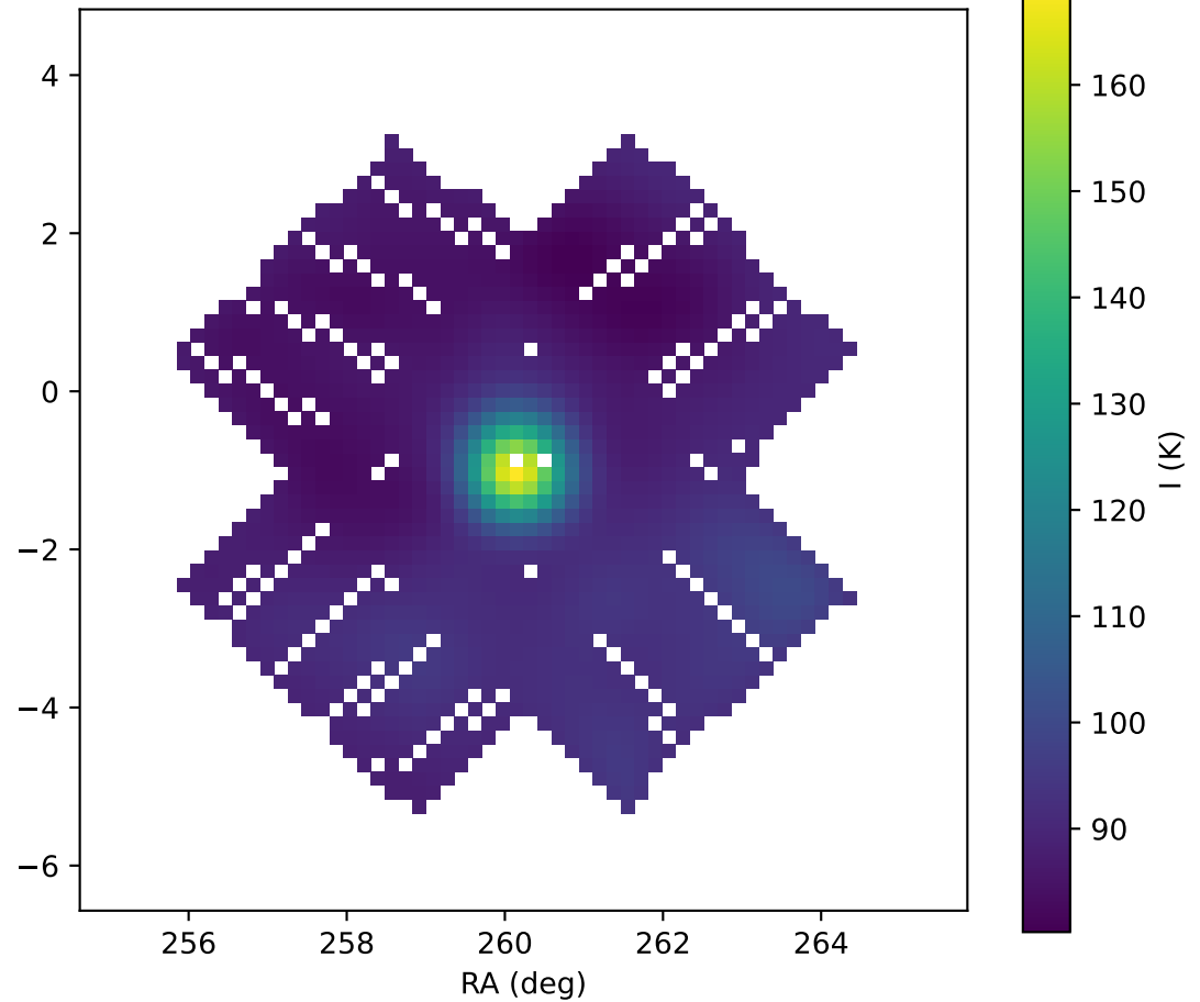
I convolved with PSF
