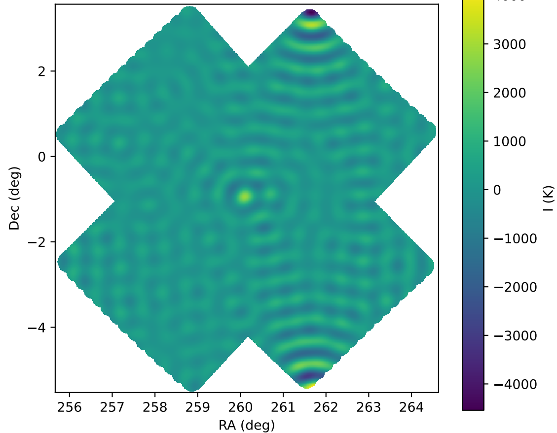
Stokes I deconvolved (Wiener)
