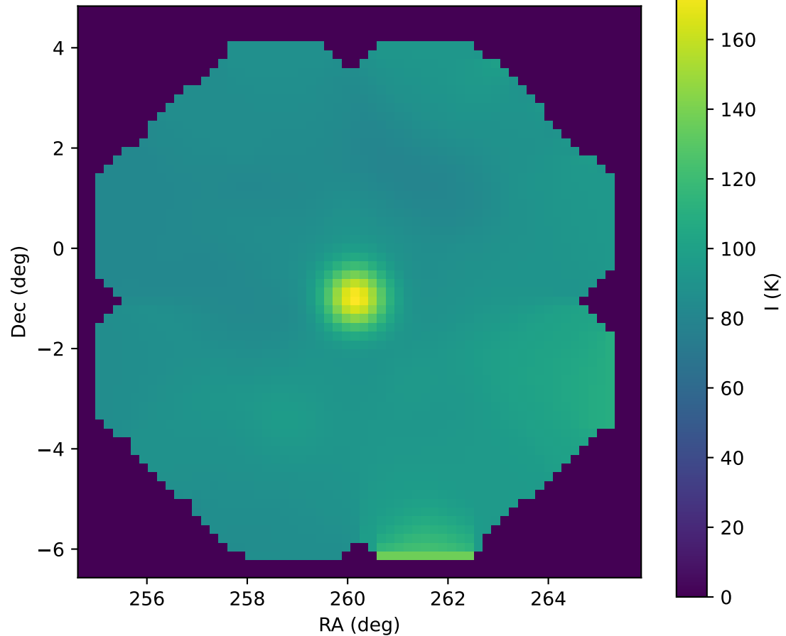
Stokes I convolved with PSF
