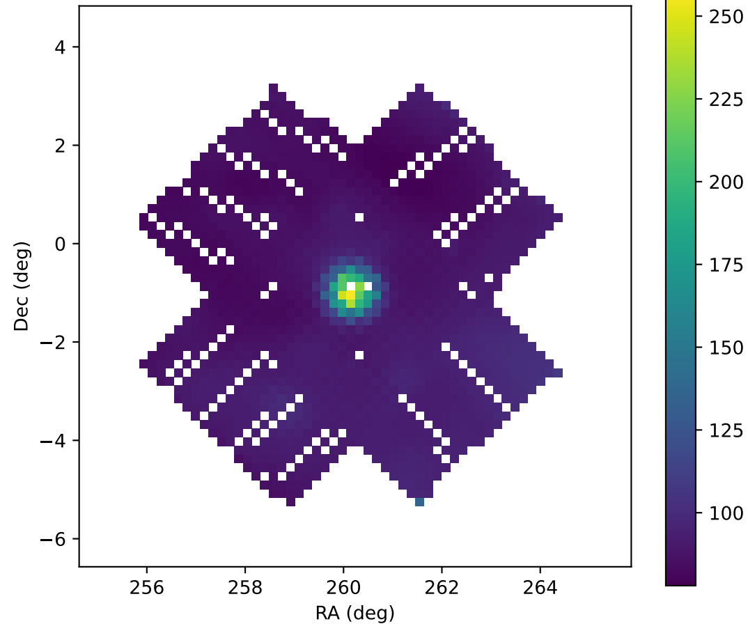
Stokes I (beam-gridded)
