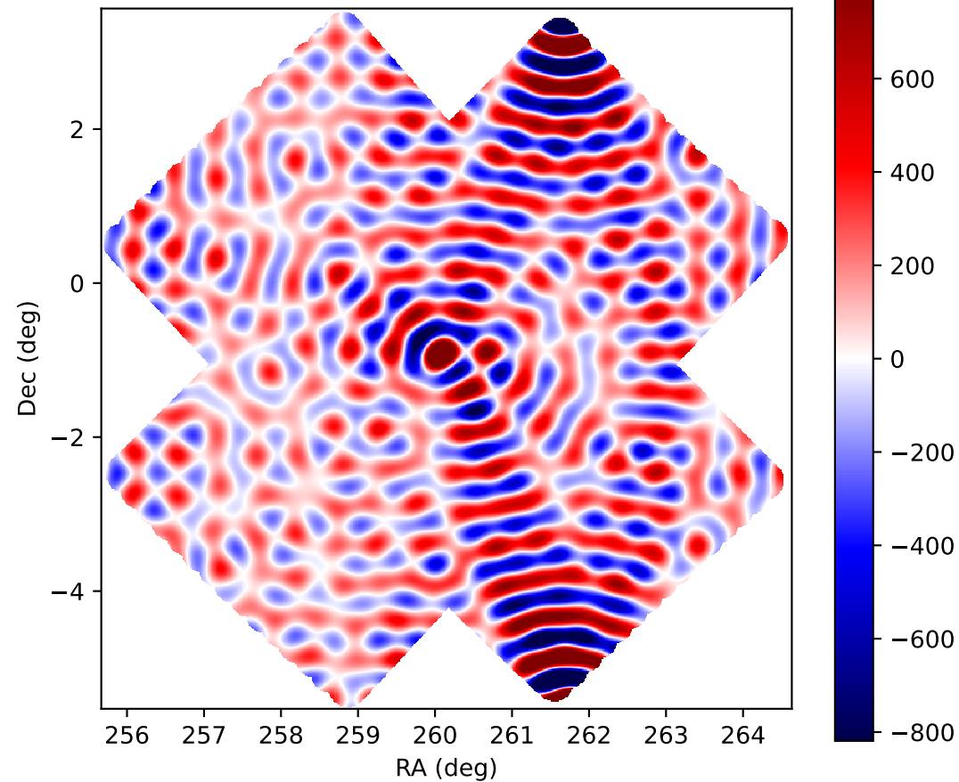
Stokes Q deconvolved (PSF removed)
