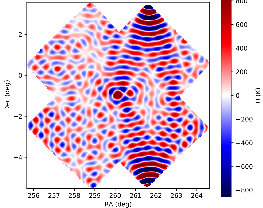
Stokes U deconvolved (PSF removed)
