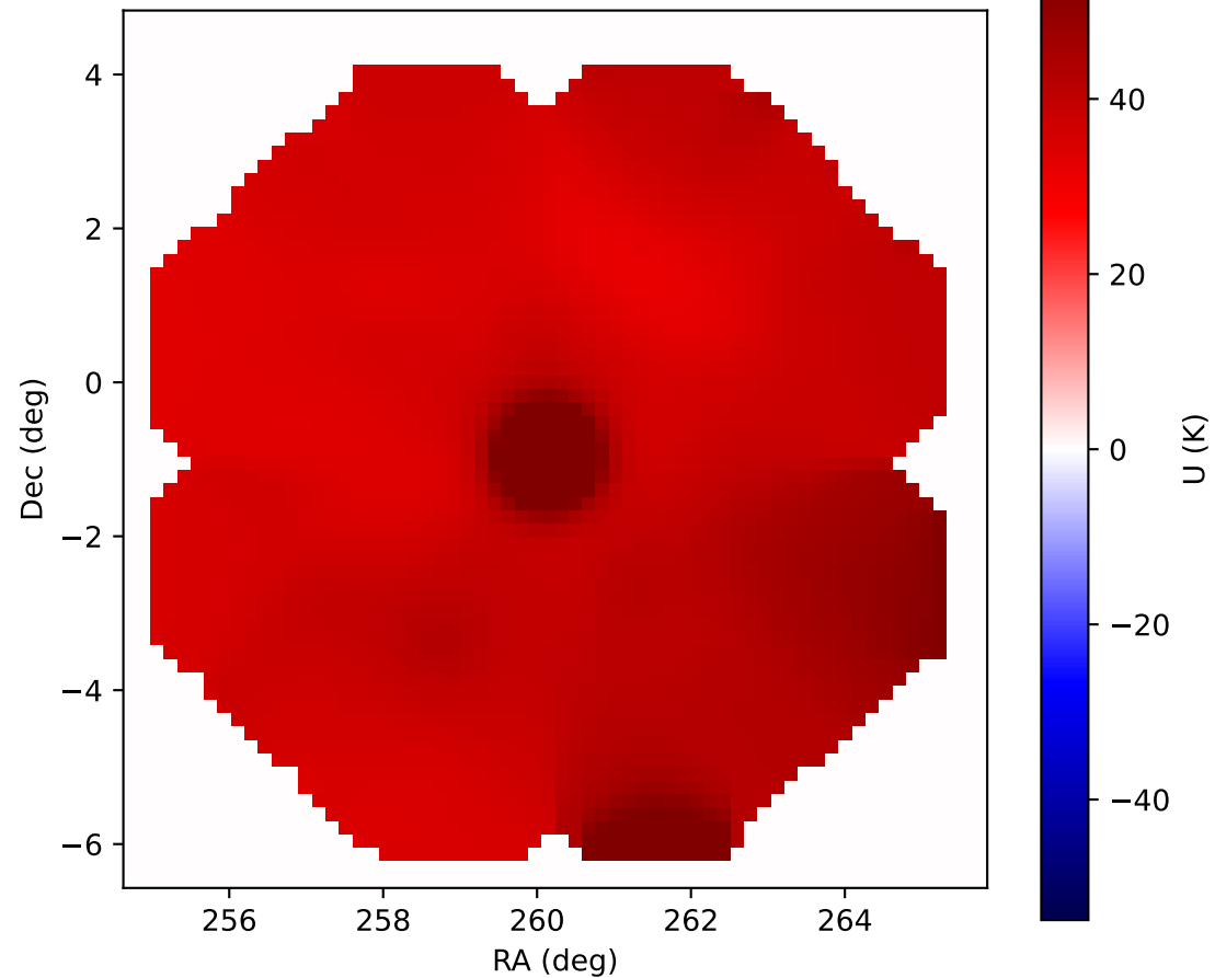
Stokes U convolved with PSF
