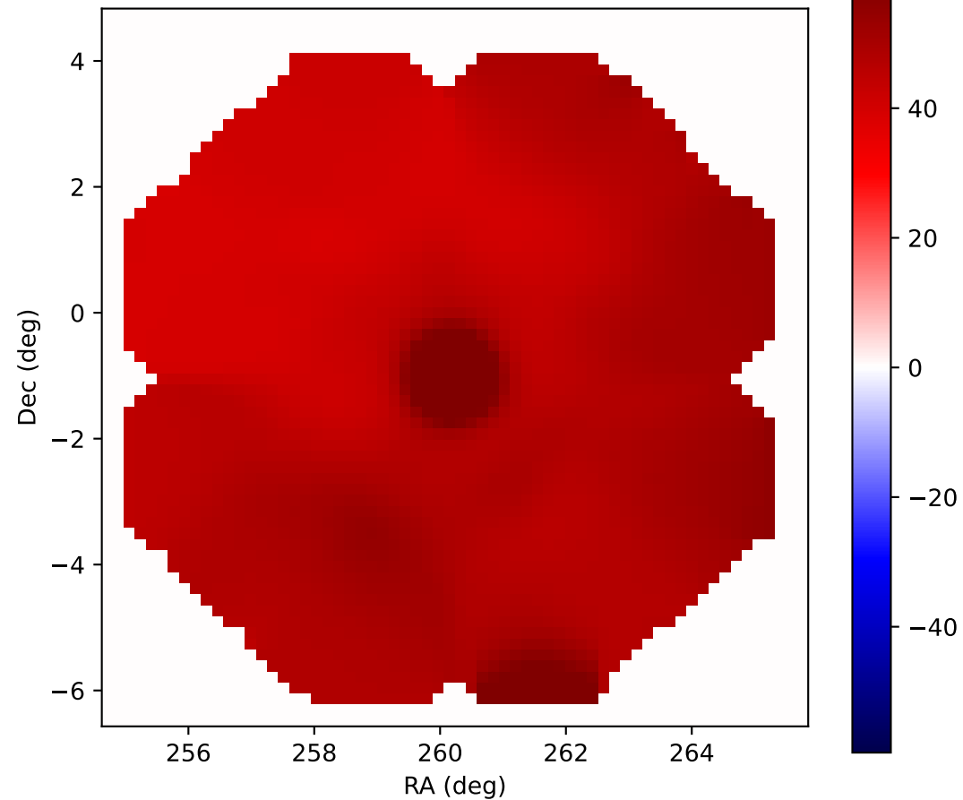
Stokes Q convolved with PSF
