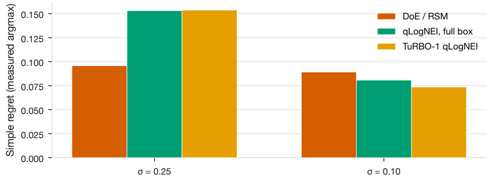
Locally constrained BO is a sampling rule, not a new readout
