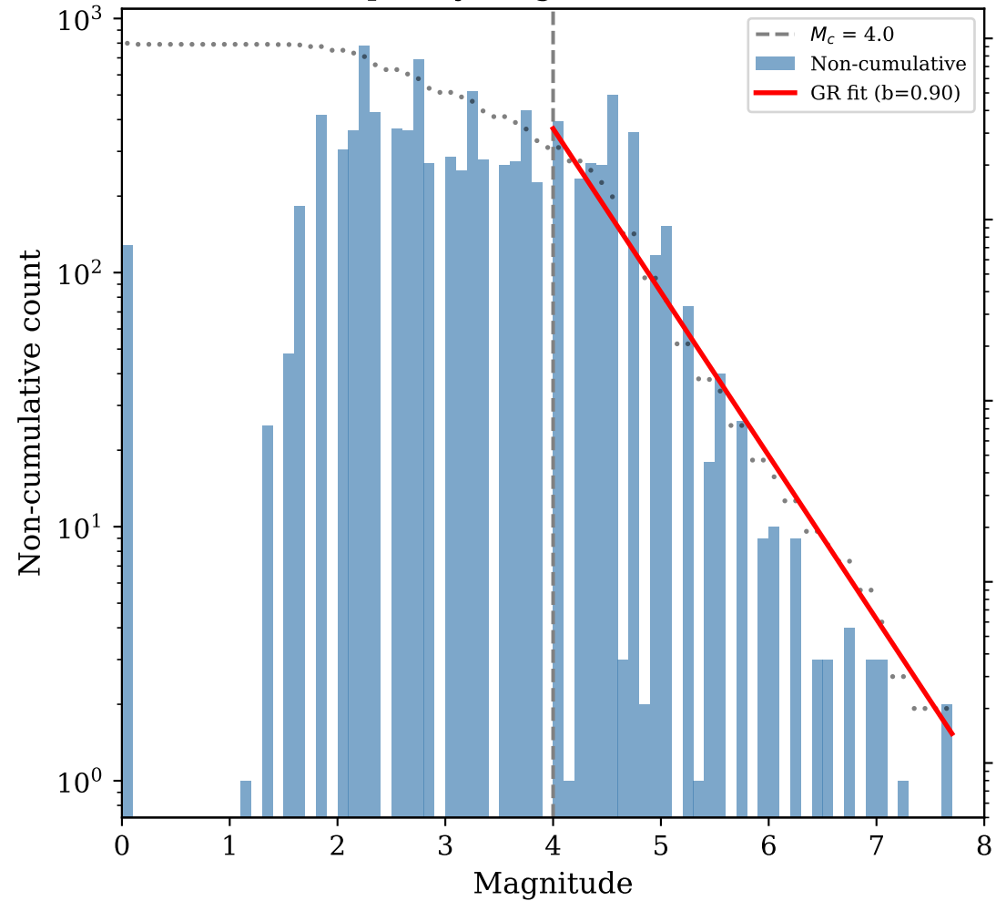
(a) Frequency-Magnitude Distribution
