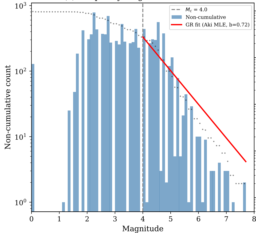
(a) Frequency-Magnitude Distribution
