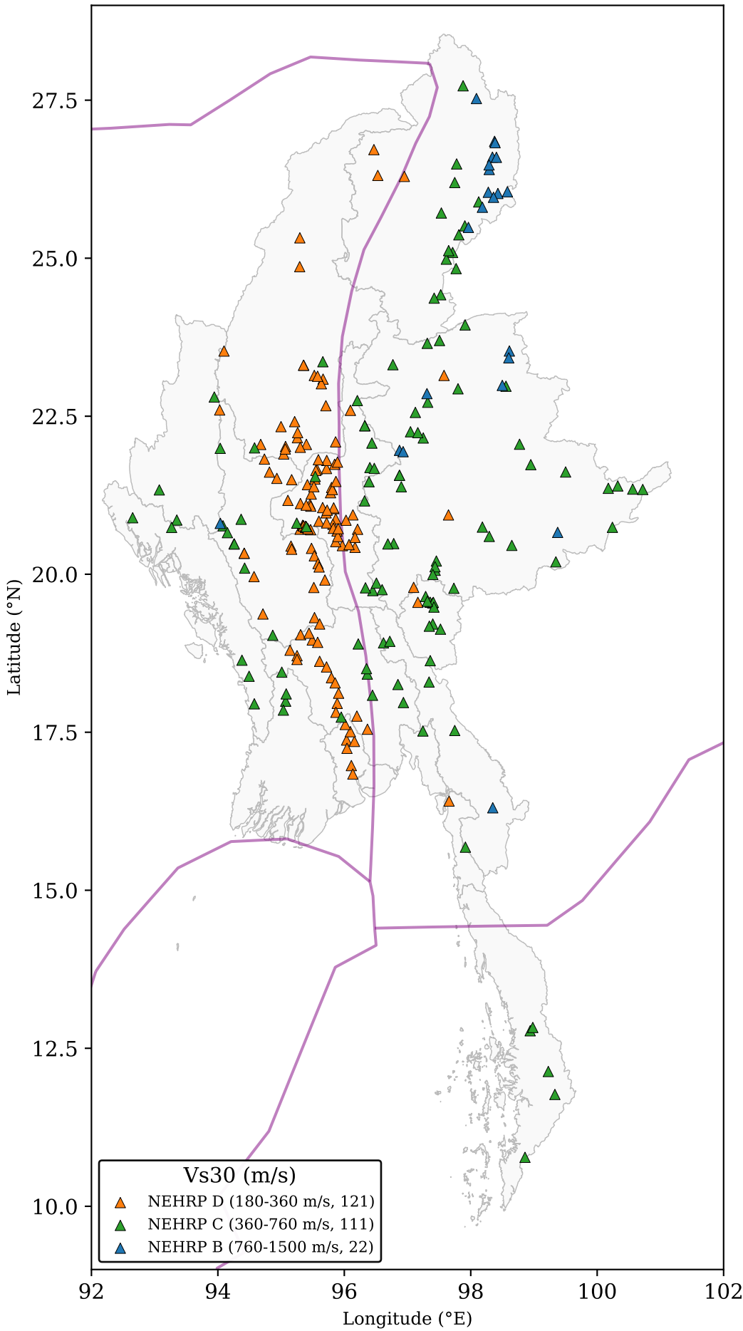
Site-Specific Vs30 at Dam Sites (Wald & Allen, 2007)
