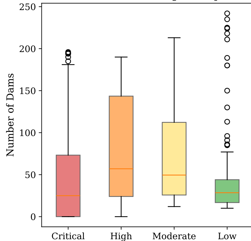
(c) Sensitivity Analysis (100 Monte Carlo weight samples)
