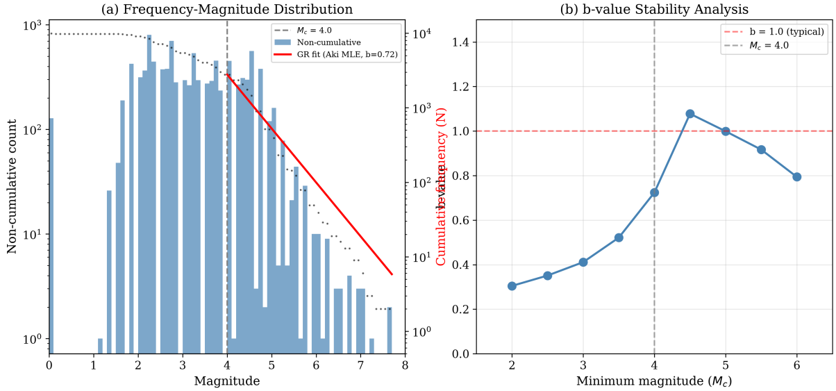
Figure 2: (a) Frequency-magnitude distribution with G-R fit above M_c = 4.0 . (b) b-value stability—it stabilizes around M_c \approx 4.0 – 4.5 , confirming the catalog is incomplete below M4. The G-R line in (a) uses the Aki (1965) MLE b-value at M_c = 4.0 , the same estimate quoted in the text.
