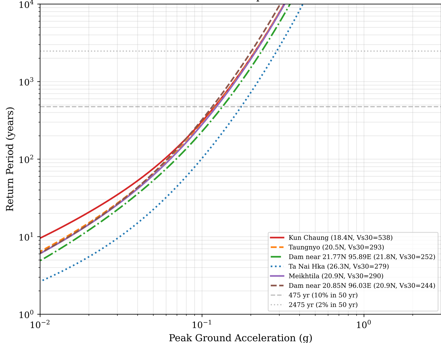
Seismic Hazard Curves at Representative Dam Sites
