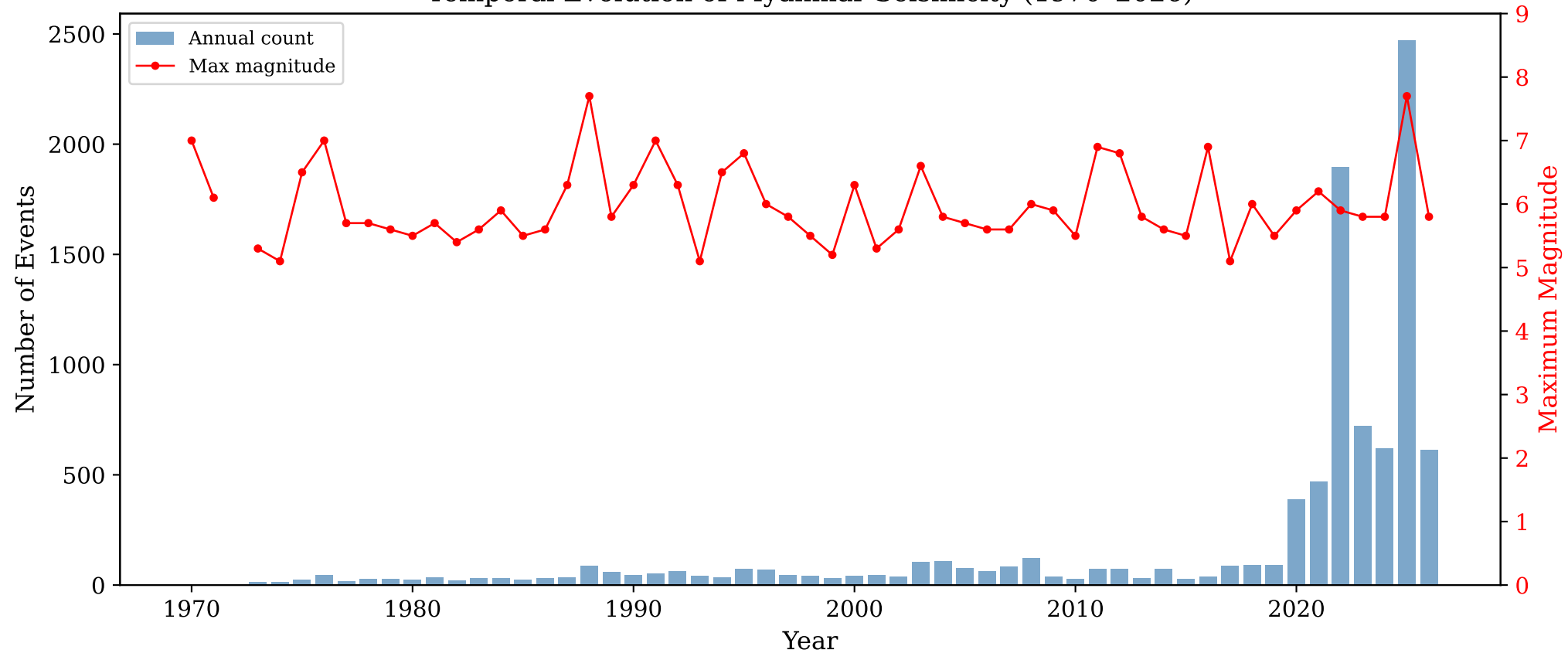
Temporal Evolution of Myanmar Seismicity (1970-2026)
