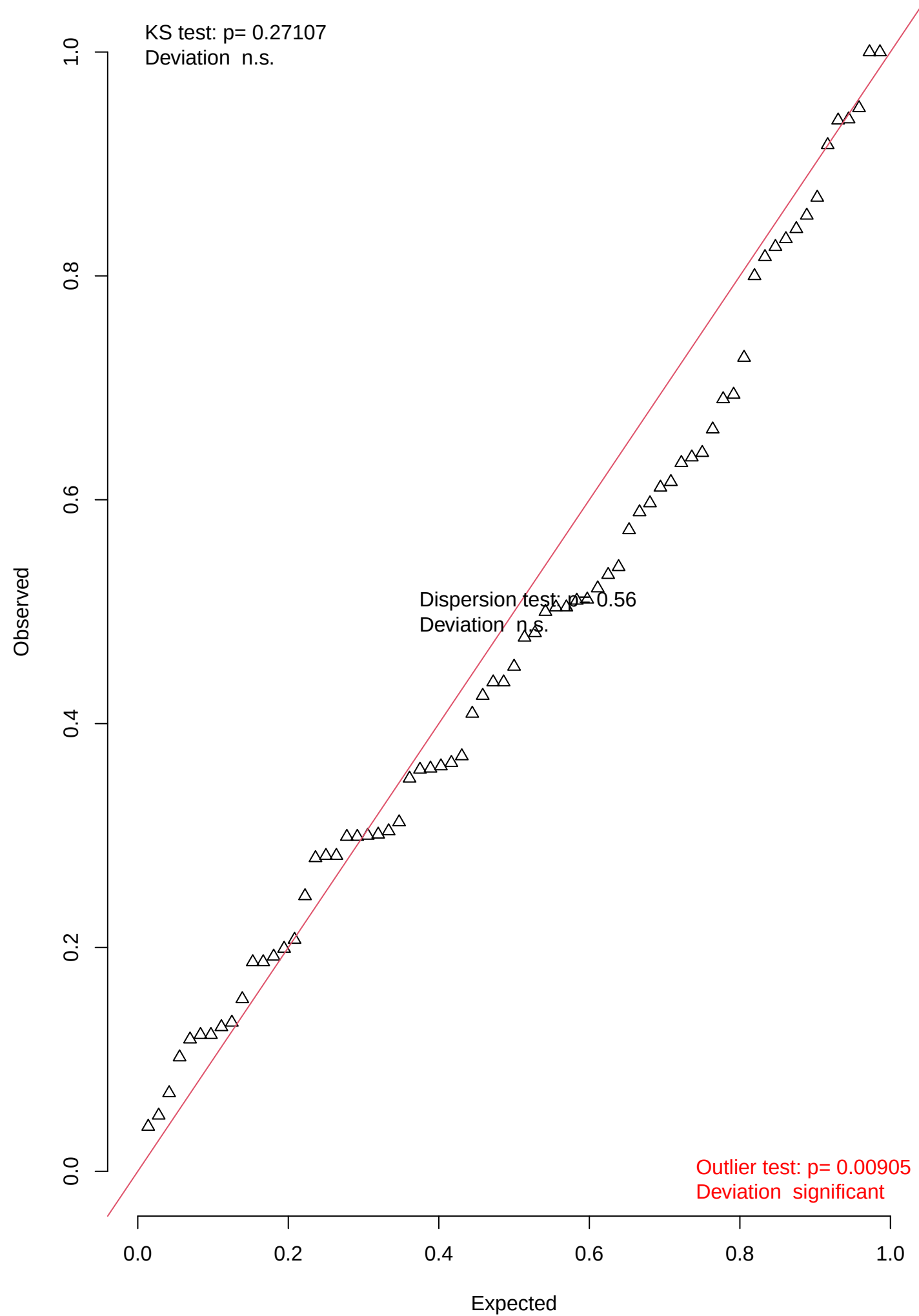
QQ plot residuals
