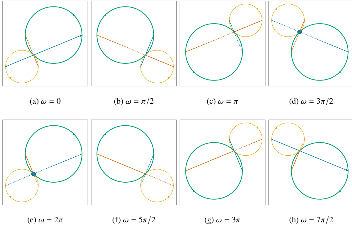
FIG. 6. 2D circle-mode projection of the z -rotation sequence from Fig. 4. The tangent circles preserve the true hyperchord radii, with their areas encoding the Born-rule probabilities.
