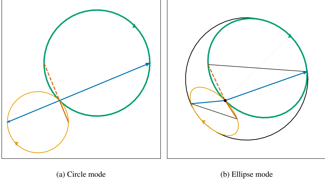
FIG. 3. Two-dimensional projection of the hyperchord visualization for the spinor \xi = [\cos(\pi/6), \sin(\pi/6)e^{i\pi/4}]^T . (a) Circle mode: the hyperchord faces are drawn as tangent circles with their true 3D radii. (b) Ellipse mode: the hyperchord faces are drawn as their orthogonal projections onto the xy -plane.
