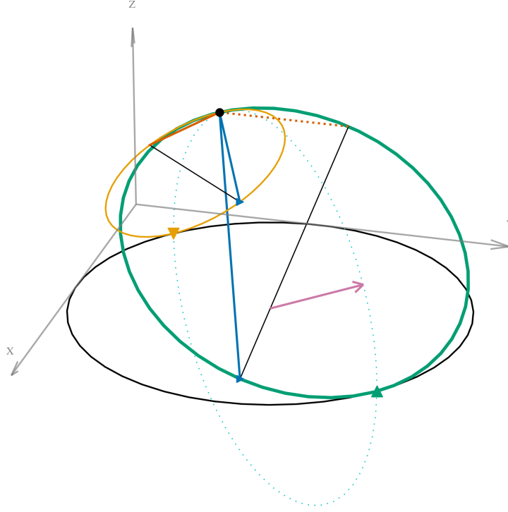
FIG. 2. Hyperchord construction. The rotated equatorial plane E' (primary datum) fixes the unit normal \mathbf{v} and the dihedral angle \vartheta with the reference plane E = xy -plane. The rotated equator e' = E' \cap S_u has a distinguished highest point Q . The two hyperchord planes U' and L' are the unique translates (through Q ) of the two dihedral-bisector planes between E and E' , with normals proportional to \mathbf{e}_z \pm \mathbf{v} . Their sphere sections are the circles c_\uparrow (teal/bluish-green, thicker line, equator contact marked with \blacktriangle ) and c_\downarrow (orange, thinner line, equator contact marked with \blacktriangledown ), with radii r_\uparrow = u \cos(\vartheta/2) and r_\downarrow = u \sin(\vartheta/2) . Each circle is tangent to the reference equator e at a unique point: P_\uparrow for c_\uparrow and P_\downarrow = -P_\uparrow for c_\downarrow . The azimuth of P_\uparrow is \varphi .
