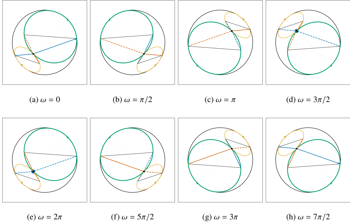
FIG. 5. 2D ellipse-mode projection of the z -rotation sequence from Fig. 4. The projected ellipses show the true orthogonal projection of the inclined hyperchord circles onto the xy -plane.
