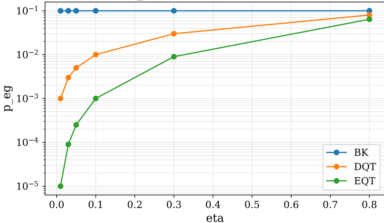
\eta \rightarrow p_{eg} mapping (distance=50 km)
