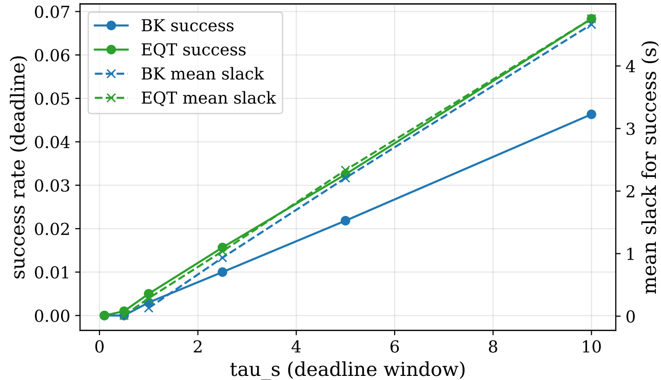
Success vs deadline window
