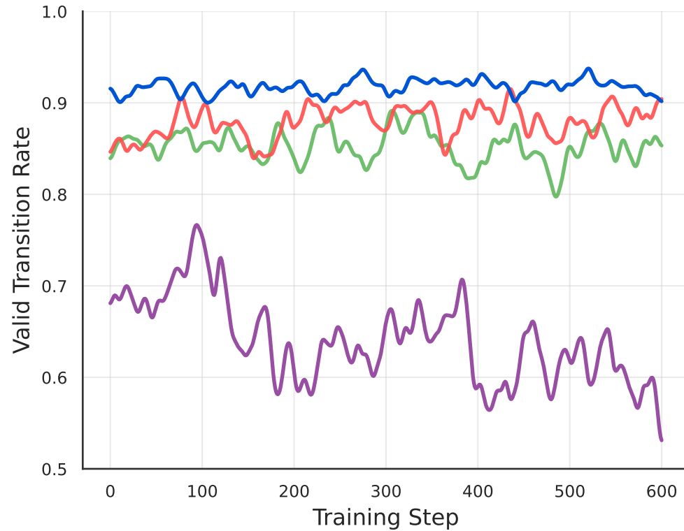
Reasoning Chain Integrity
