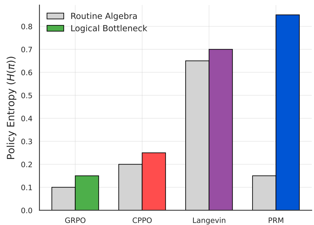
Targeted Exploration Policy Entropy
