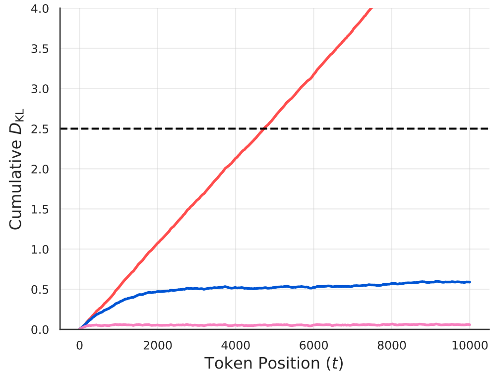
Prefix KL Divergence K_t (Single Sequence)
