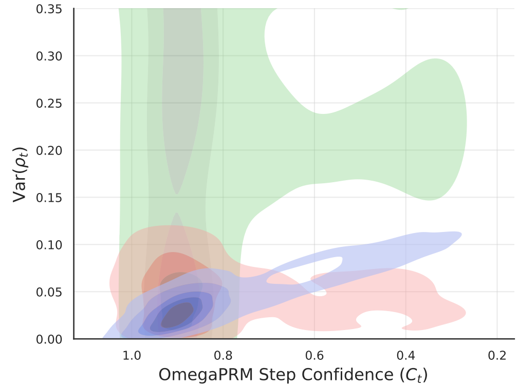
Density: Variance vs. Logic Confidence
