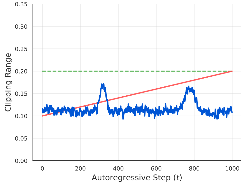
Trust Region Bound ( \varepsilon_t )
