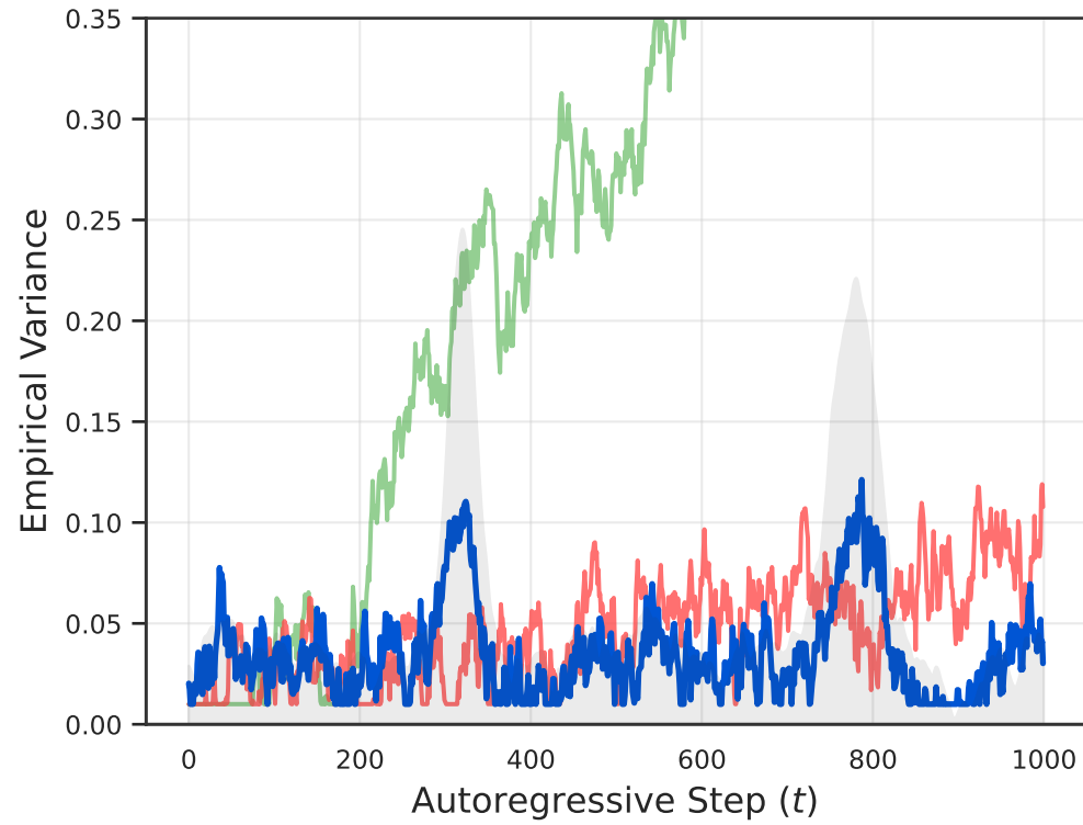
IS Ratio Variance ( \text{Var}(\rho_t) )
