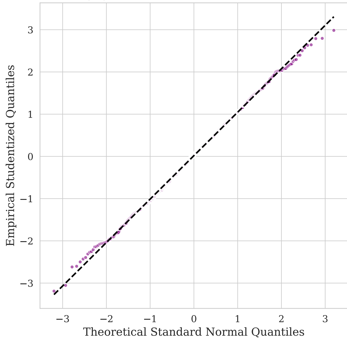
Q-Q Plot of the Debiased Estimator
