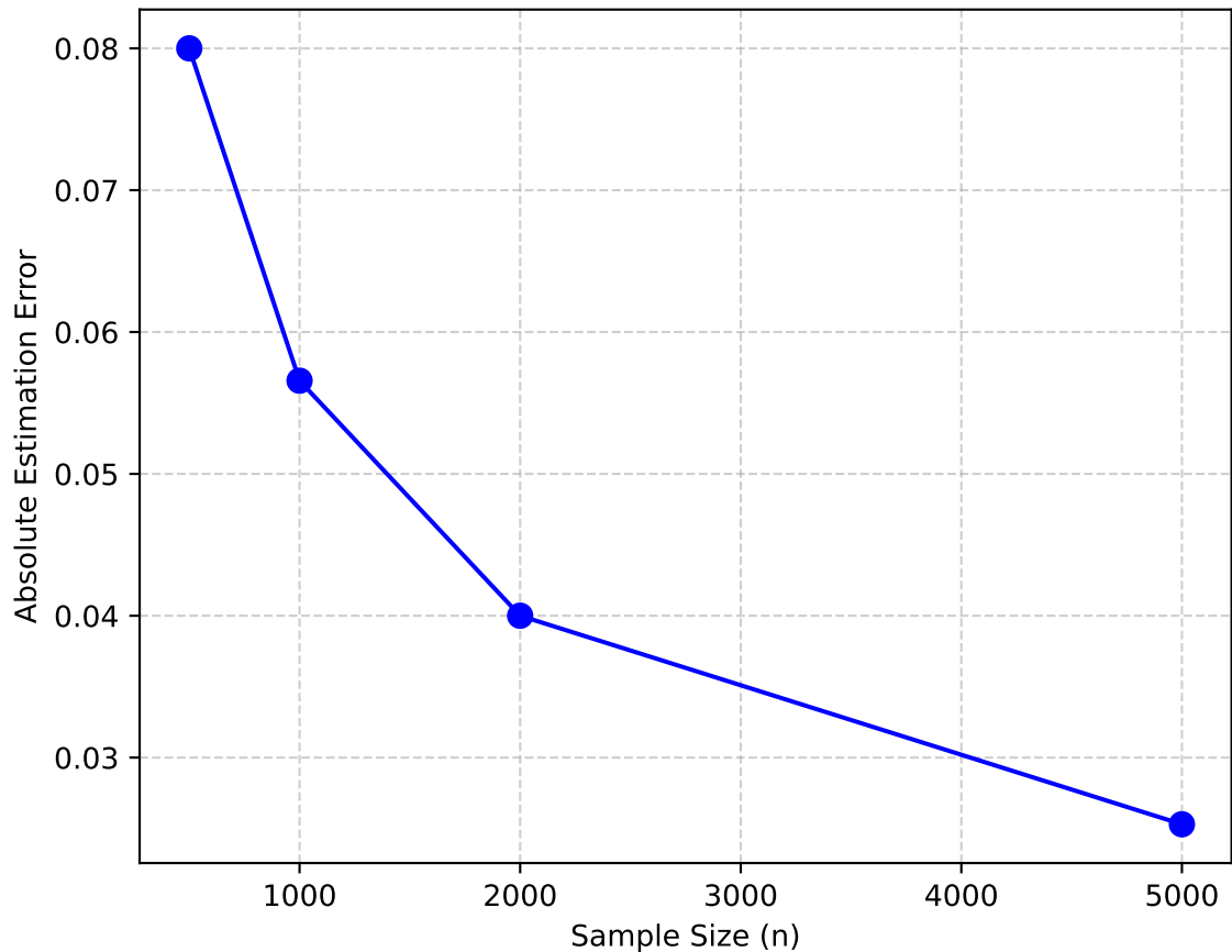
Reward Estimation Error vs. Sample Size
