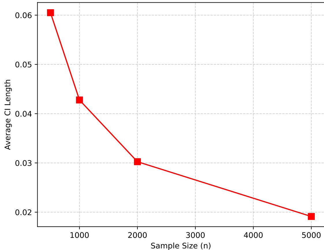
Confidence Interval Length vs. Sample Size
