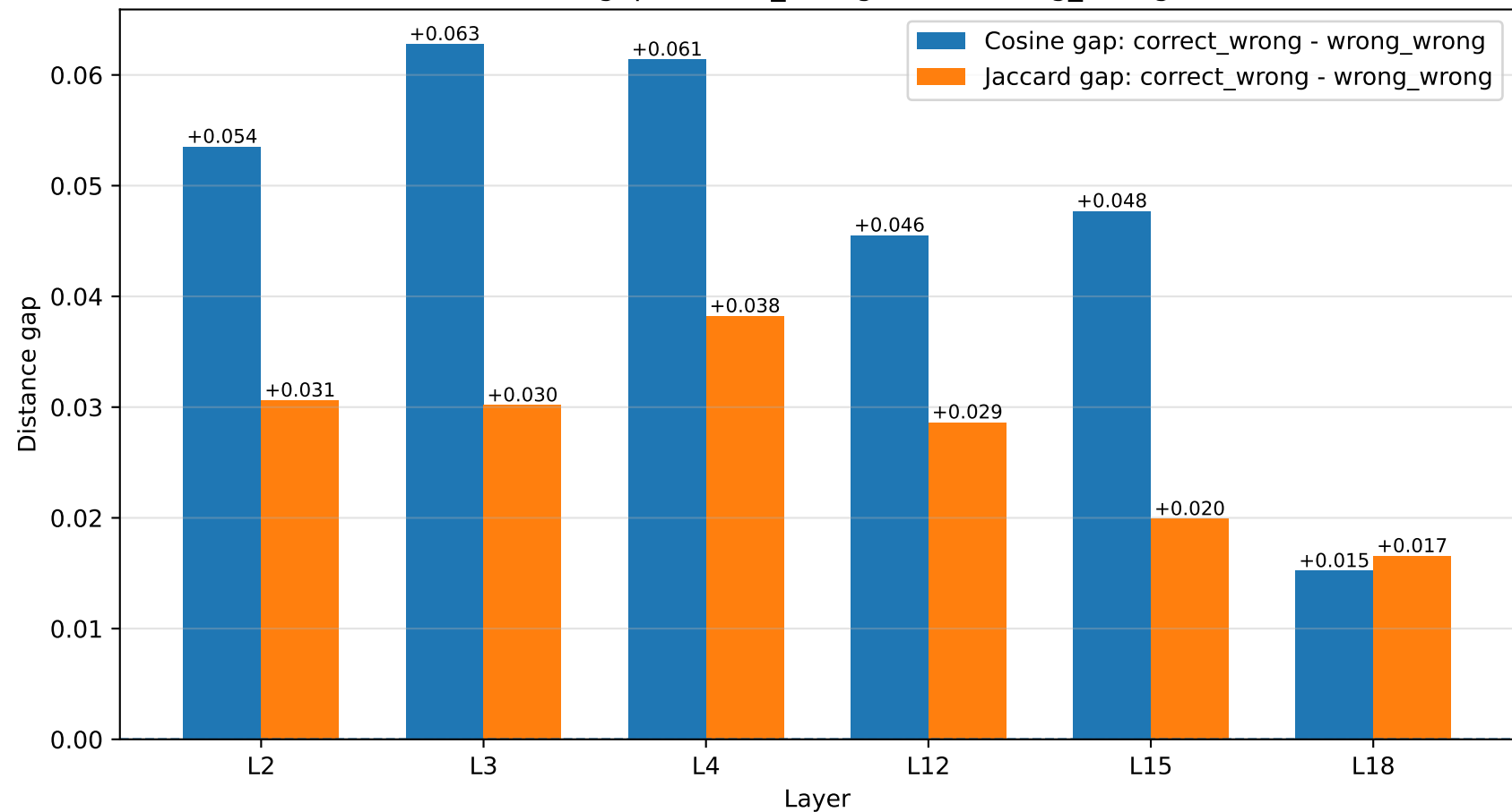
Distance gap: correct_wrong minus wrong_wrong
