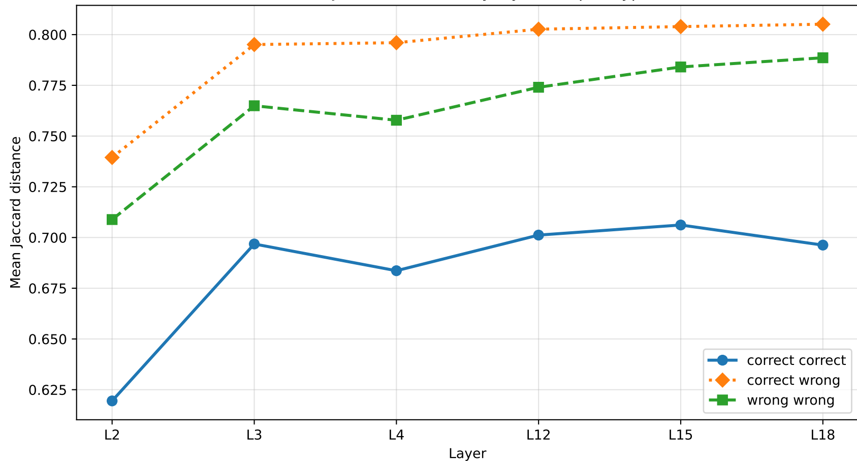
Mean Jaccard distance by layer and pair type
