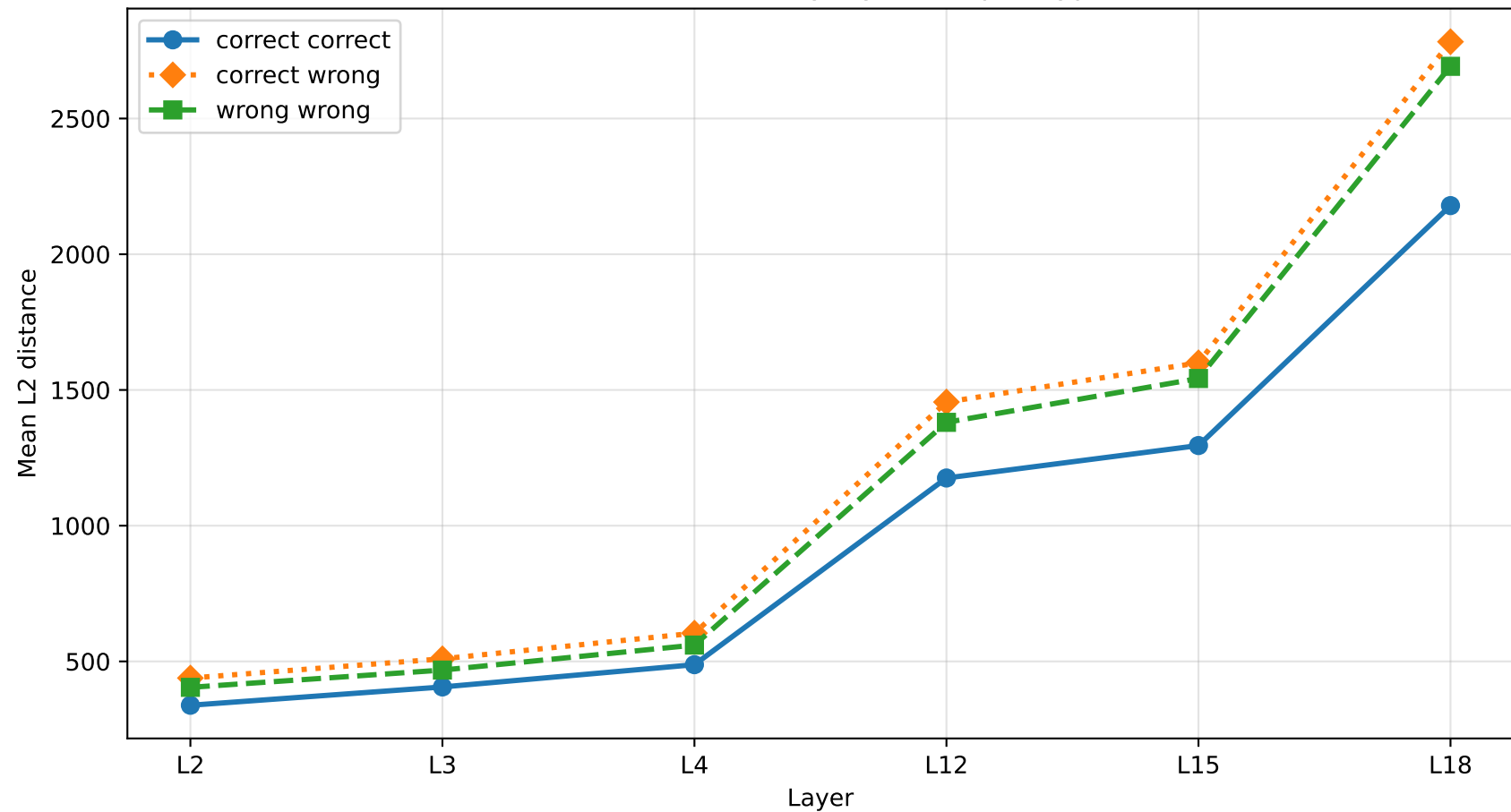
Mean L2 distance by layer and pair type
