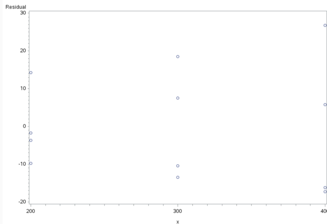
Residual Plot for Machine Speed vs Number of Defectives Checking for Unequal Error Variance (Ch. 11 Concept)
