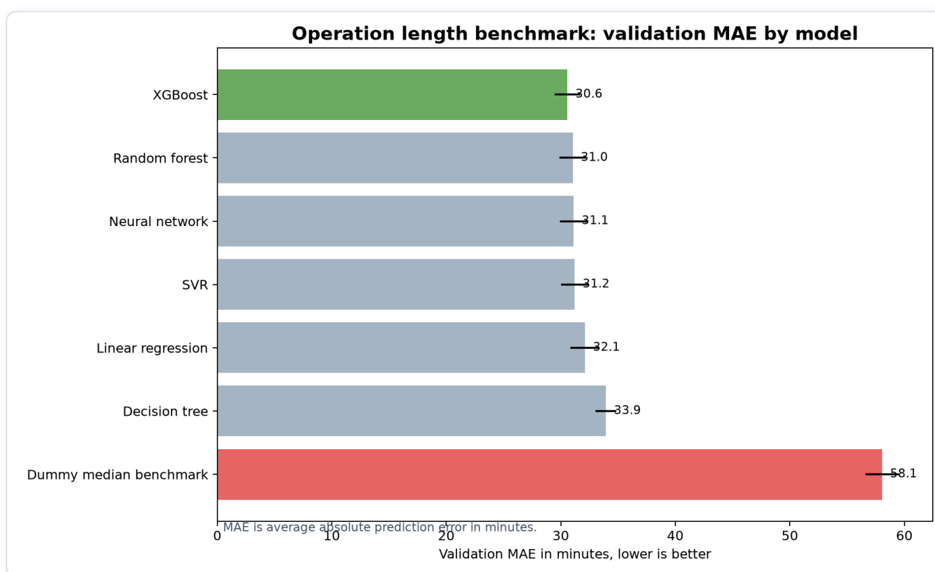
Figure 9. Model MAE benchmark. Compares MAE in minutes; lower is better. Source: operation length modelling notebook.
