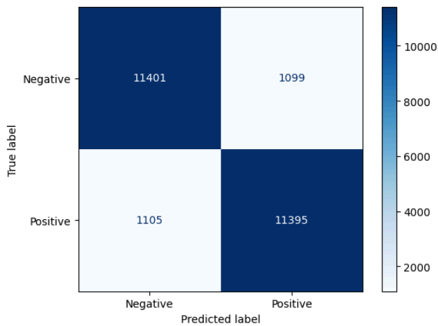
Figure 13: Fine-Tuned RoBERTa Confusion Matrix
