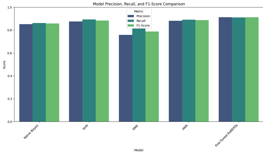
Figure 15: Models' Precisions, Recalls and F1-Scores
