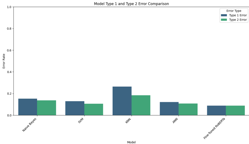
Figure 17: Models' Type 1 Errors & Type 2 Errors
