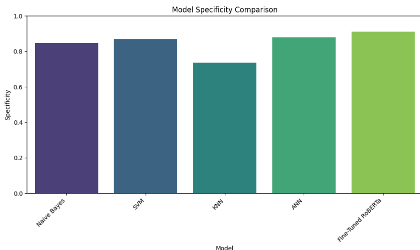
Figure 16: Models' Specificities
