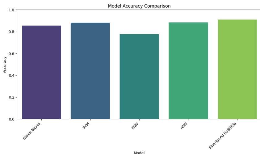
Figure 14: Models' Accuracies
