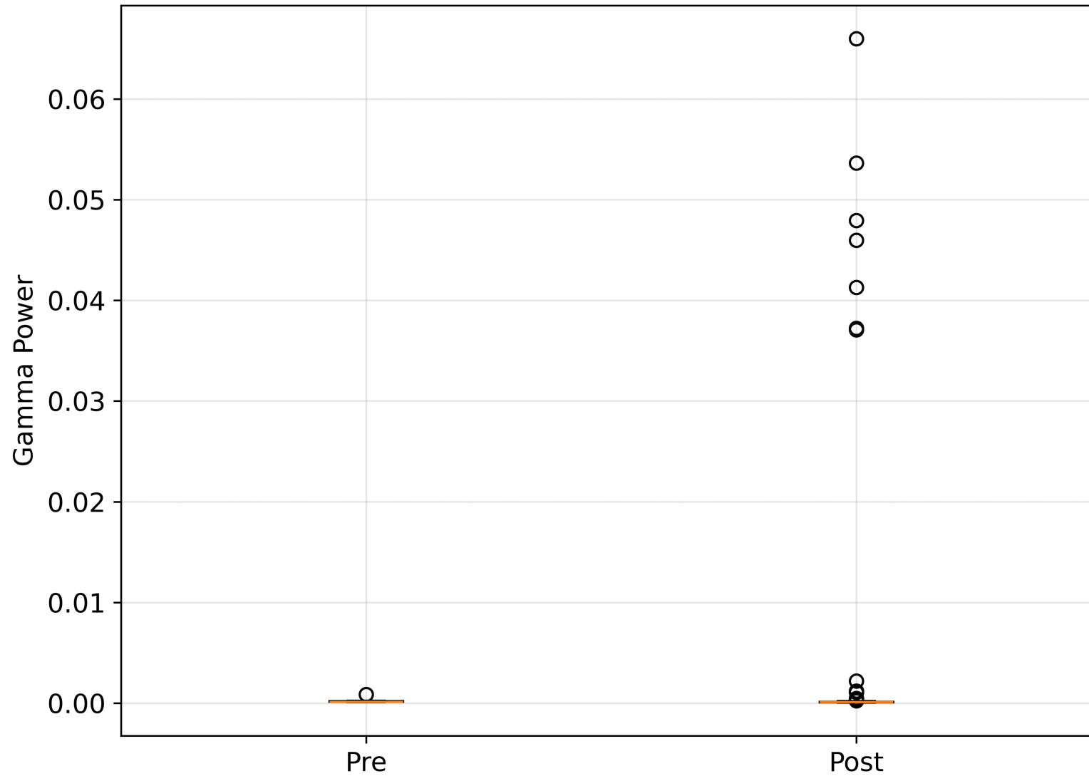
08. Gamma 40-50 Hz Pre/Post t \approx 72.059082 s (Perm p=0.7682 )
