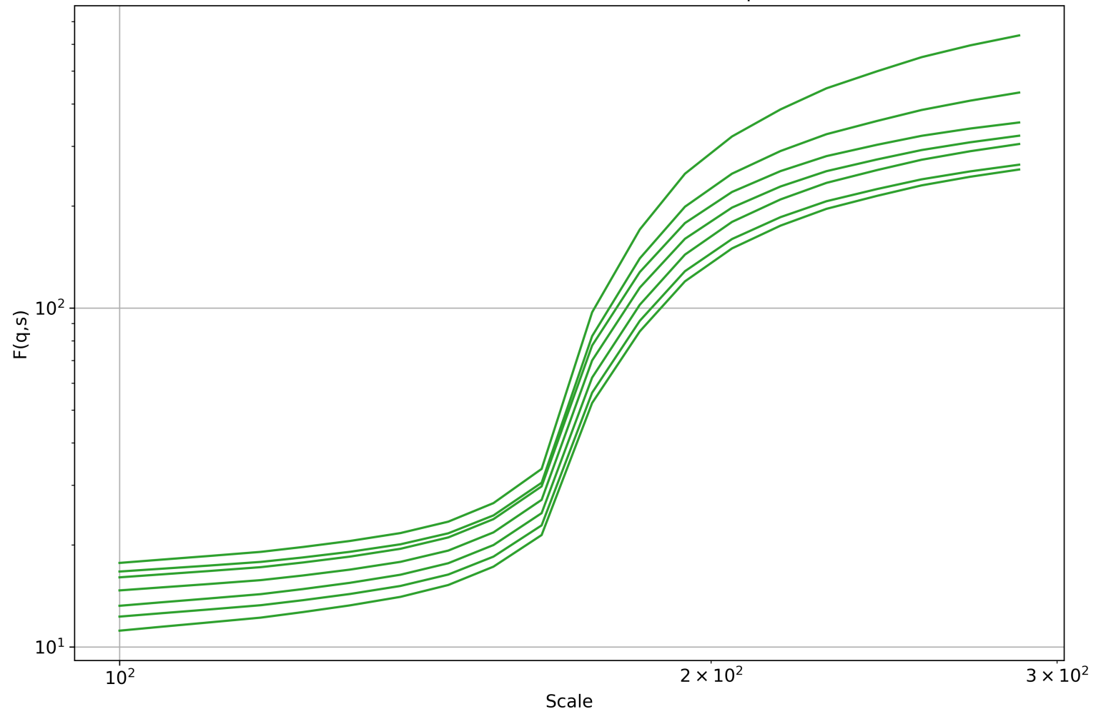
19. MFDFA on Izhikevich Network Output
