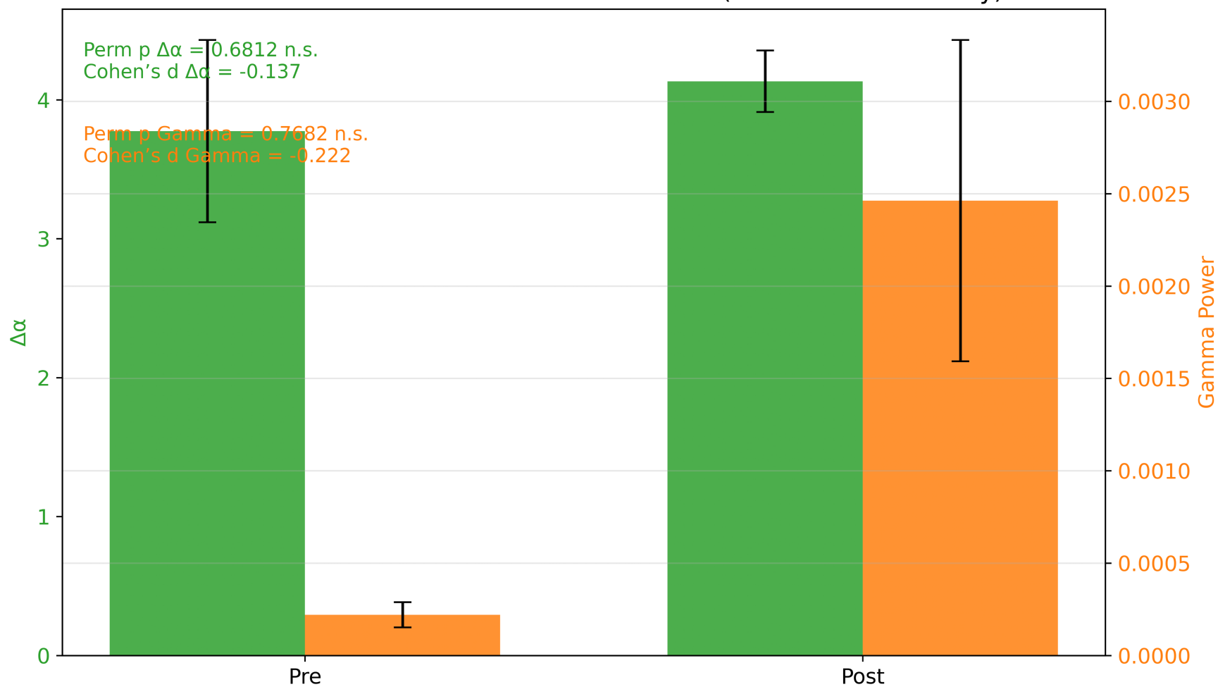
29. \Delta\alpha and Gamma Power Pre vs Post t \approx 41 s (Main Effect Summary)
