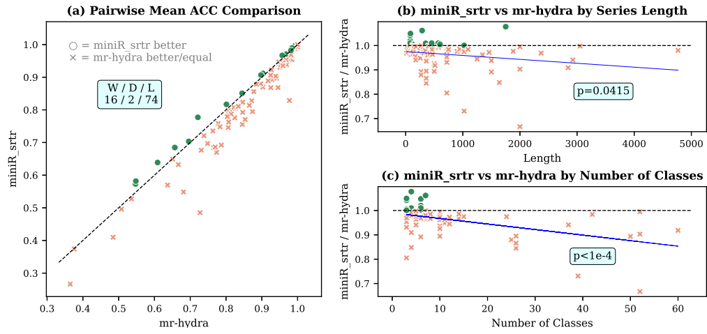
Fig. S4. Performance comparison of miniR_srtr versus mr-hydra: (a) mean accuracy values, and how miniR_srtr's advantage correlates with (b) series length and (c) number of classes, quantified by Pearson correlation.
