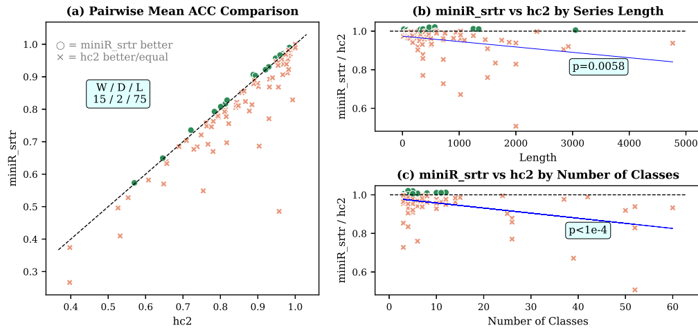
Fig. S3. Performance comparison of miniR_srtr versus hc2: (a) mean accuracy values, and how miniR_srtr's advantage correlates with (b) series length and (c) number of classes, quantified by Pearson correlation.
