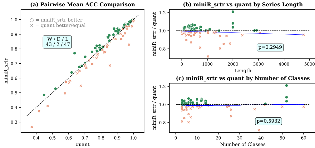
Fig. S1. Performance comparison of miniR_srttr versus quant: (a) mean accuracy values, and how miniR_srttr’s advantage correlates with (b) series length and (c) number of classes, quantified by Pearson correlation.
