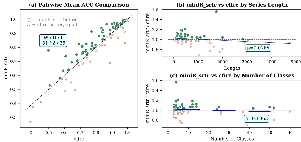
Fig. S2. Performance comparison of miniR_srttr versus cfire: (a) mean accuracy values, and how miniR_srttr’s advantage correlates with (b) series length and (c) number of classes, quantified by Pearson correlation.
