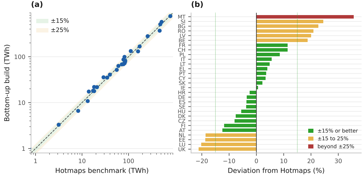
Figure S1: Bottom-up demand reconstruction against the Hotmaps top-down surface. Per country (a), on log axes with \pm 15 and \pm 25 per cent guide bands, and as the percentage deviation (b).
