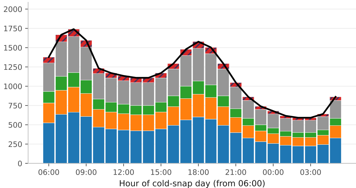
Heat (GW-thermal)
