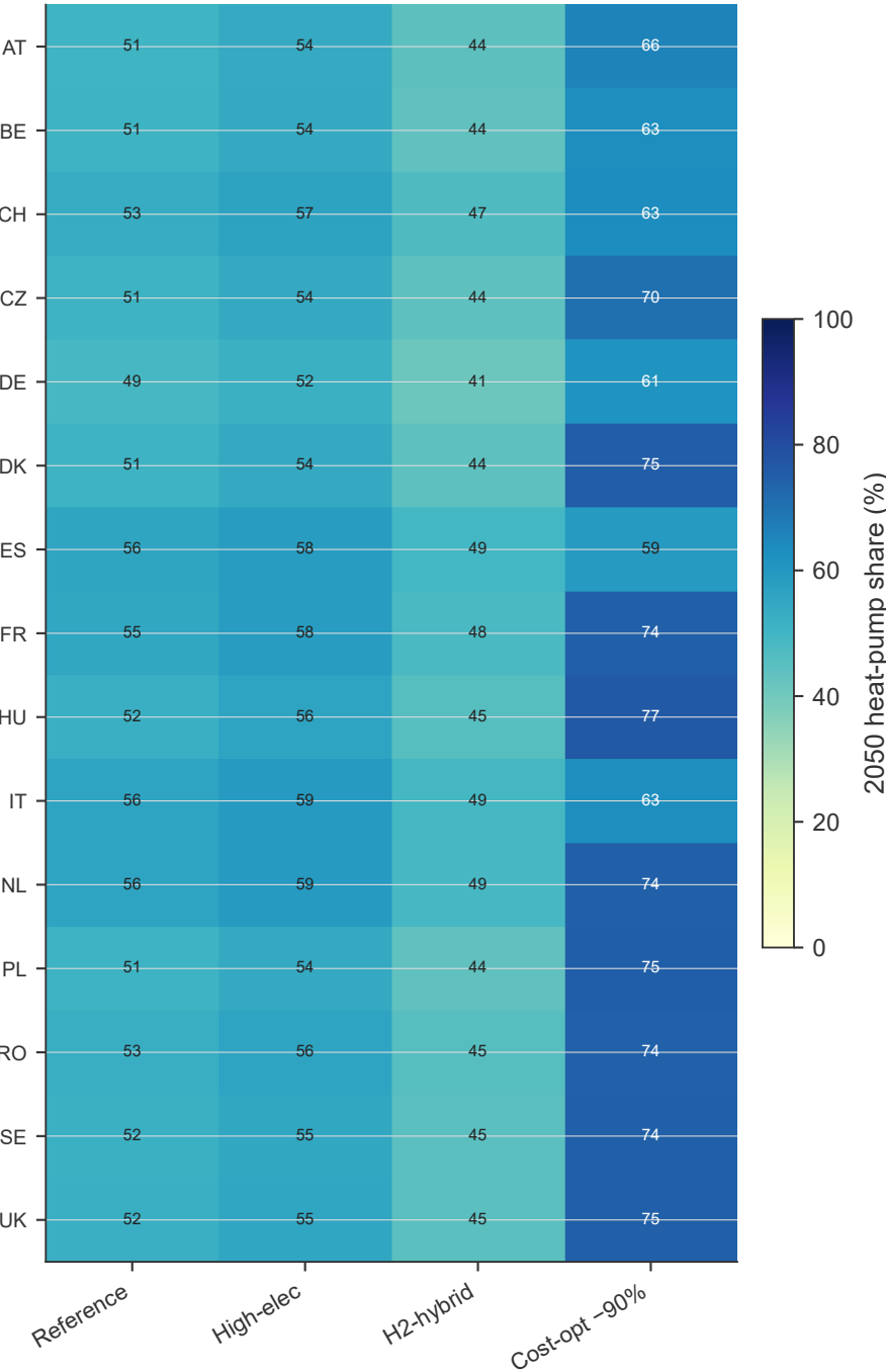
2050 heat-pump share by country and scenario
