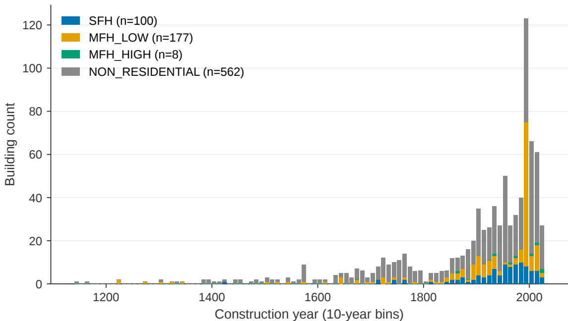
Construction-year distribution of the 847 buildings with year metadata
