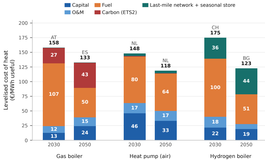
Figure 4: Levelised cost of heat by component, 2030 and 2050. The market at the study median for each technology and year, named above its bar. Air-source heat pump.
