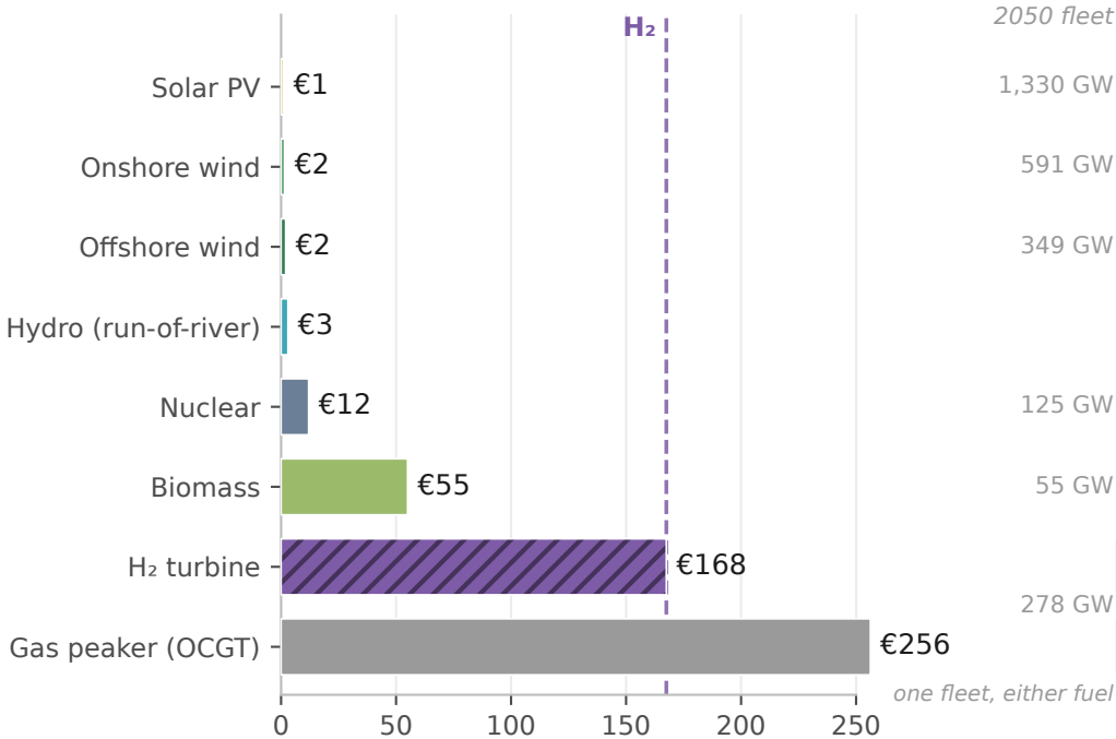
Short-run marginal cost, 2050 (€/MWh-e), fuel and carbon only
