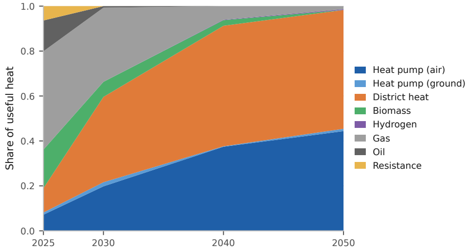
Figure B.1: The EU least-cost heating pathway under the -90 per cent scope-1 cap. Each band is a technology’s share of EU useful heat, so the vertical axis runs from 0 to 1 and the bands sum to it in every year. Hydrogen carries a band of 0.3 per cent, which is not visible at this scale, and that absence is the figure’s point.
