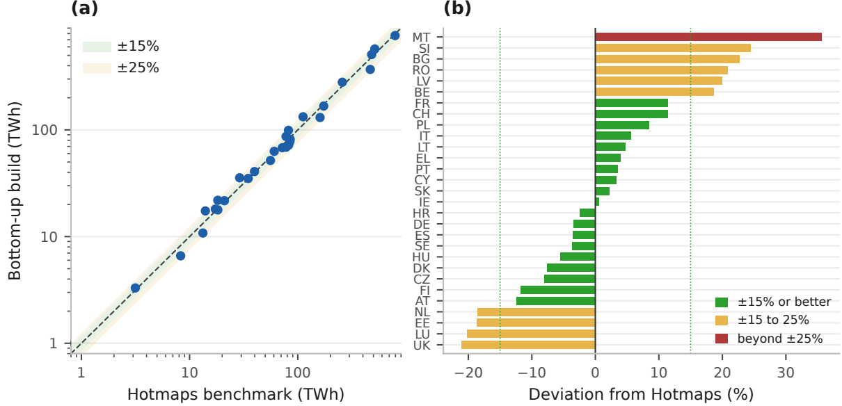
Figure A.1: Validation of the bottom-up build against the Hotmaps baseline. Panel (a) plots each country’s bottom-up demand against its Hotmaps benchmark on log axes, with the dashed line parity and the shaded bands \pm 15 and \pm 25 per cent. Panel (b) gives the same deviation per country as a sorted bar chart, coloured green inside \pm 15 per cent, amber to \pm 25 and red beyond.
